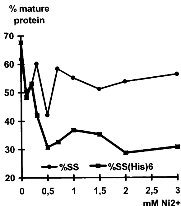
Fig. 4. Quantitative estimation of the inhibition of pSS(His) 6 import into isolated chloroplasts at increasing \text{Ni}^{2+} concentration. The amount of radioactivity in the mature and precursor protein band of Fig. 3 was measured using a PhosphorImager. The amount of mature protein is represented in percent of the sum of mature and precursor protein.
