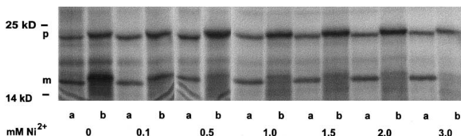
Fig. 3. Effect of increasing \text{Ni}^{2+} concentrations on the chloroplast import of pSS and pSS(His) 6 . Composite picture of three fluorograms of a 10–20% polyacrylamide gel with electrophoretically separated incubation mixtures. Each lane was loaded with an equal amount of chlorophyll a+b . Isolated chloroplasts were incubated in the presence of the indicated \text{Ni}^{2+} concentrations with in vitro synthesized, radiolabeled pSS (lanes a) or pSS(His) 6 (lanes b). p, precursor protein; m, mature protein.
